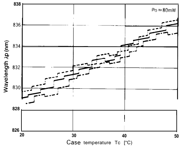
Fig. 90-4 Wavelength vs. Temperature
