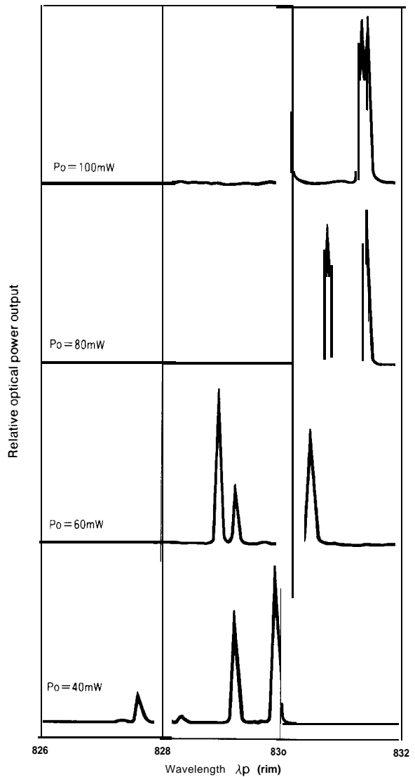
Fig. 90-5 Optical Power Output Dependence of Wavelength
