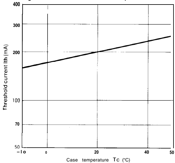
Fig. 90-3 Threshold Current vs. Temperature
